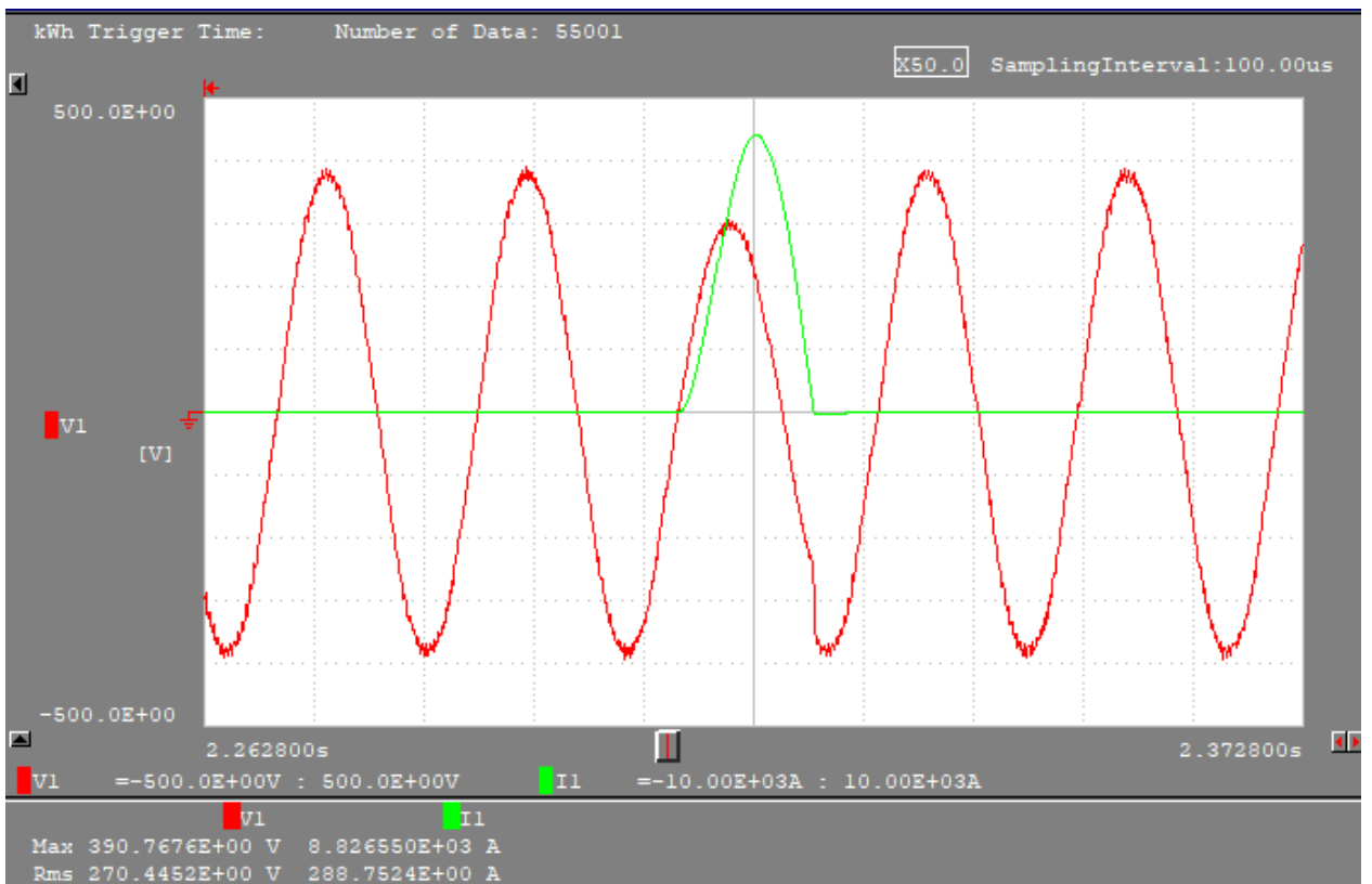
Figure 10: plot of measured test shot 3, for C6 test 1, short-circuit current carrying capacity
