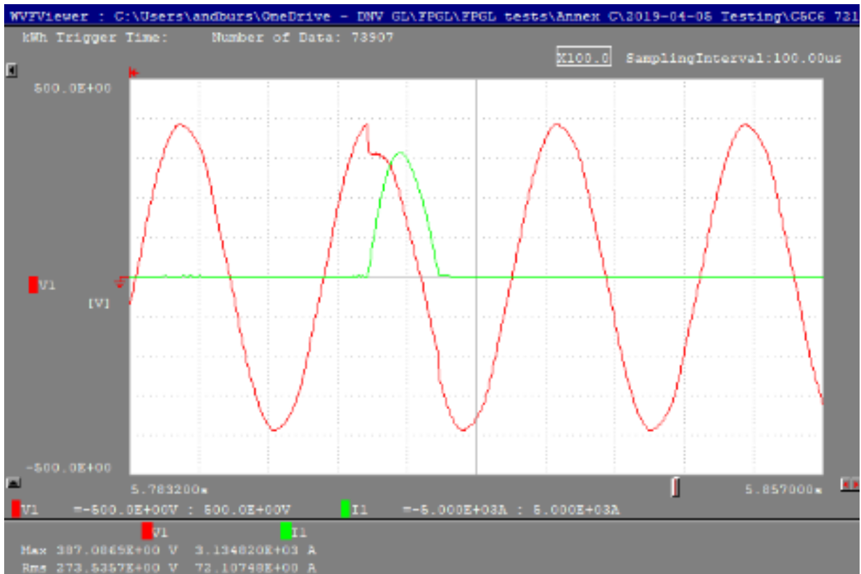
Figure 4: plot of measured test shot 1, for C5, fault current making capacity
