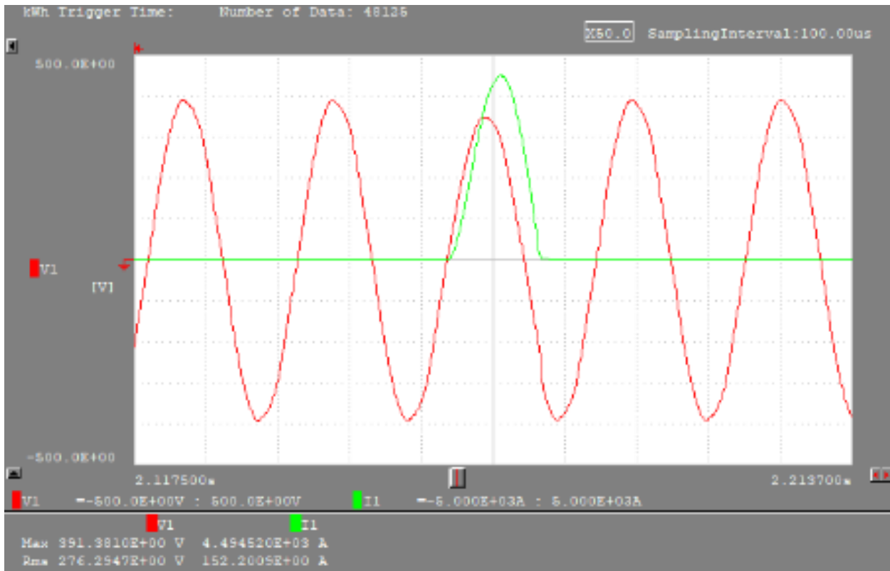
Figure 13: plot of measured test shot 2, for C6 test 2, short-circuit current carrying capacity
