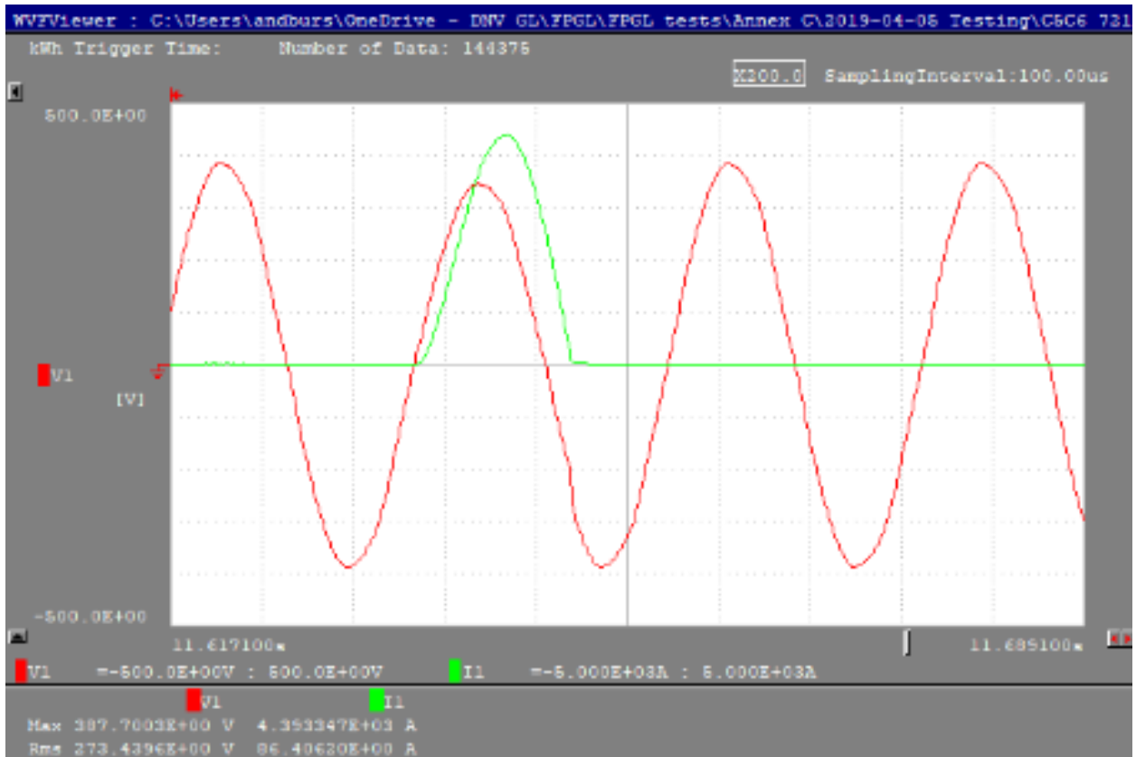
Figure 5: plot of measured test shot 2, for C5, fault current making capacity
