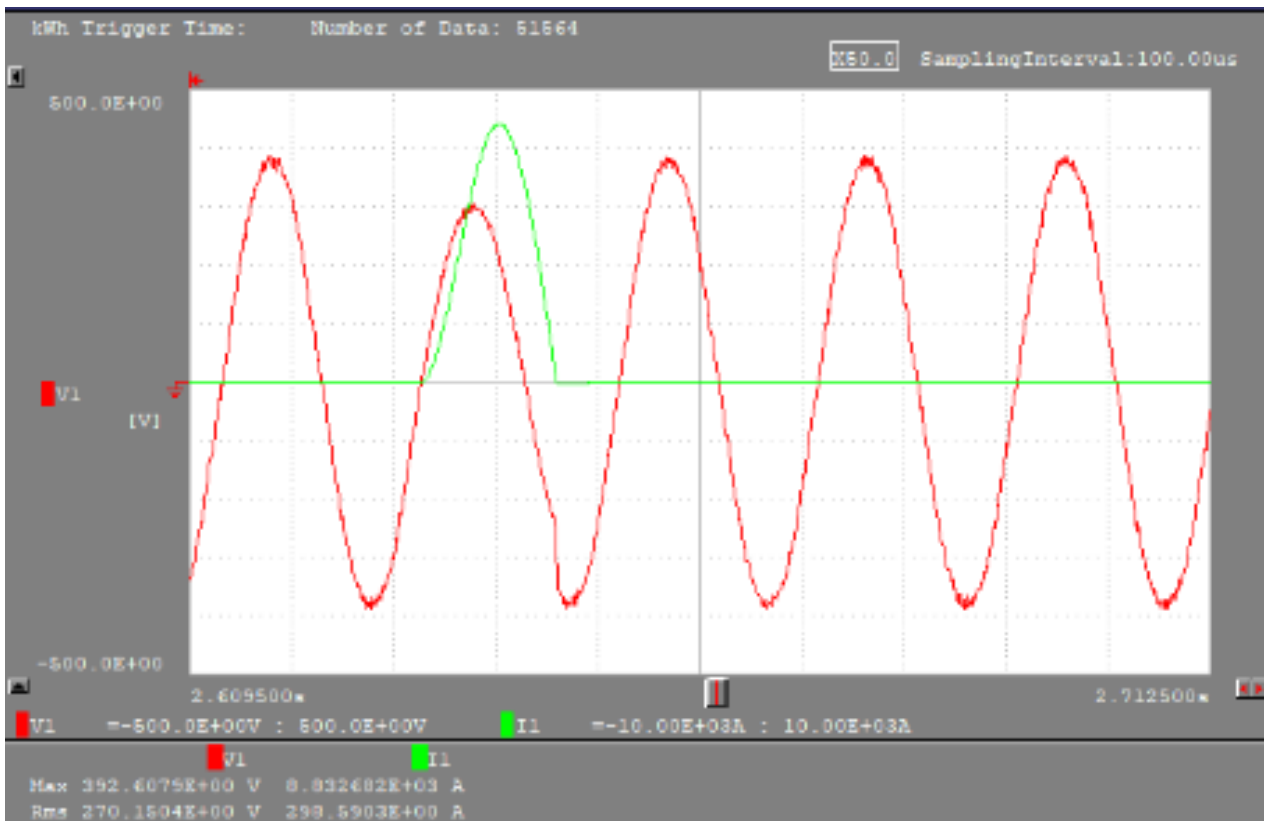
Figure 9: plot of measured test shot 2, for C6 test 1, short-circuit current carrying capacity
