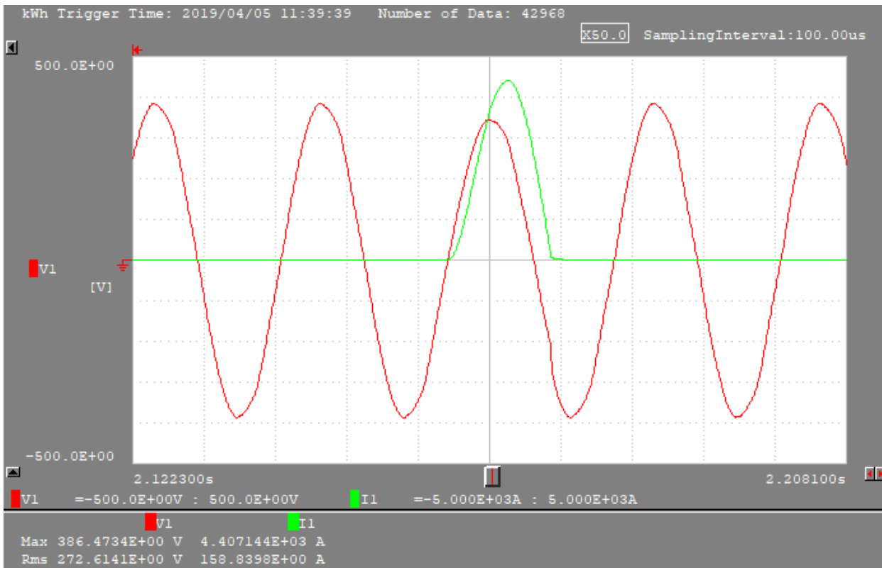
Figure 3: plot of measured initial test shot for C5, fault current making capacity
