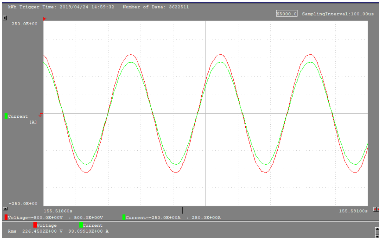
Figure 1: plot of first cycle from C3, to indicate electrical quantities at PF=1
