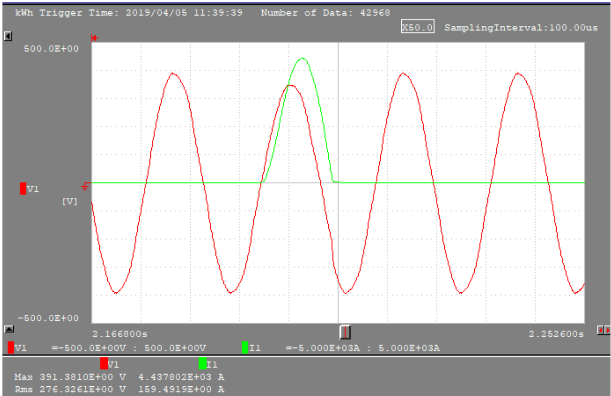
Figure 11: plot of measured initial test shot for C6 test 2, short-circuit current carrying capacity
