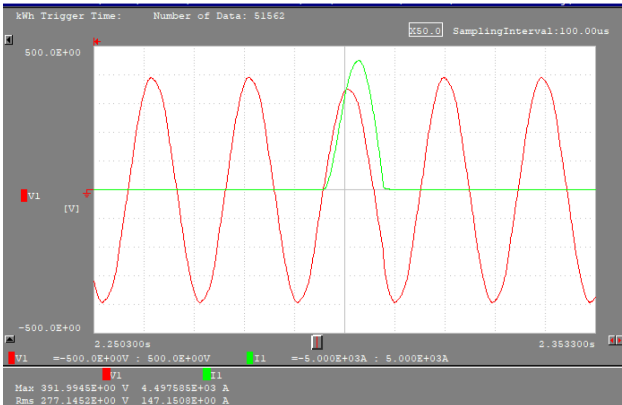
Figure 14: plot of measured test shot 3, for C6 test 2, short-circuit current carrying capacity
