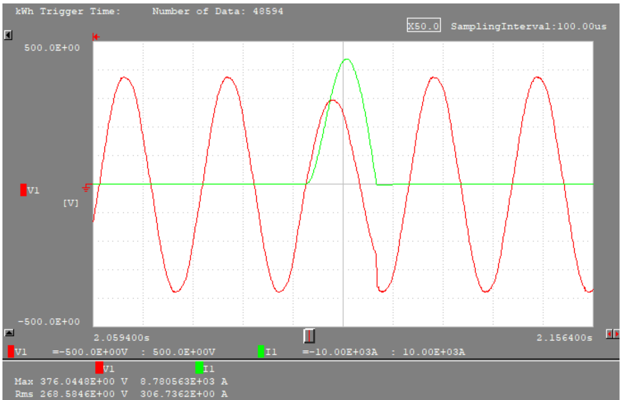
Figure 7 plot of measured initial test shot for C6 test 1, short-circuit current carrying capacity
