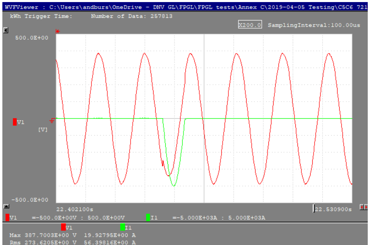
Figure 6: plot of measured test shot 3, for C5, fault current making capacity
