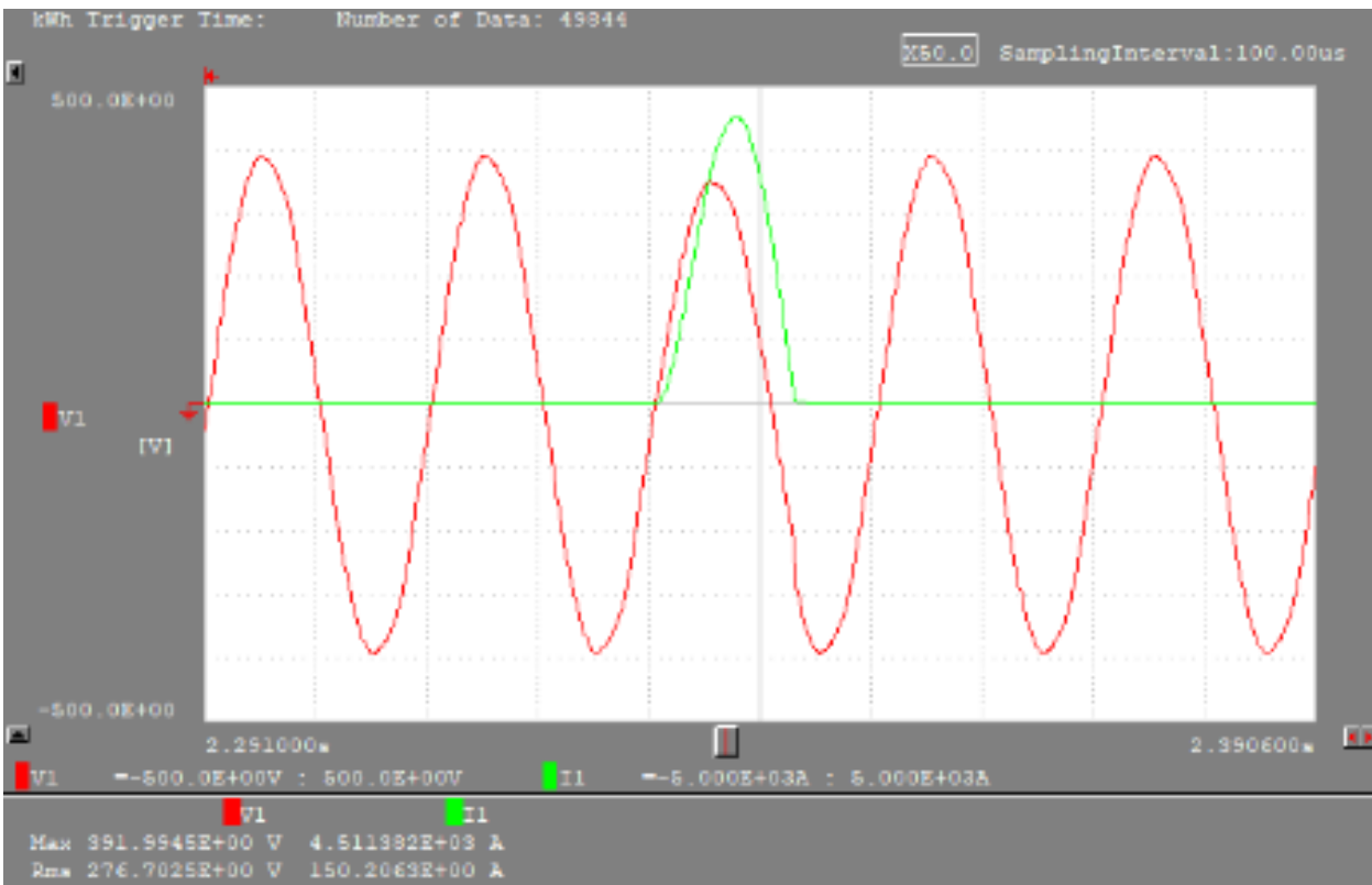
Figure 12: plot of measured test shot 1, for C6 test 2, short-circuit current carrying capacity
