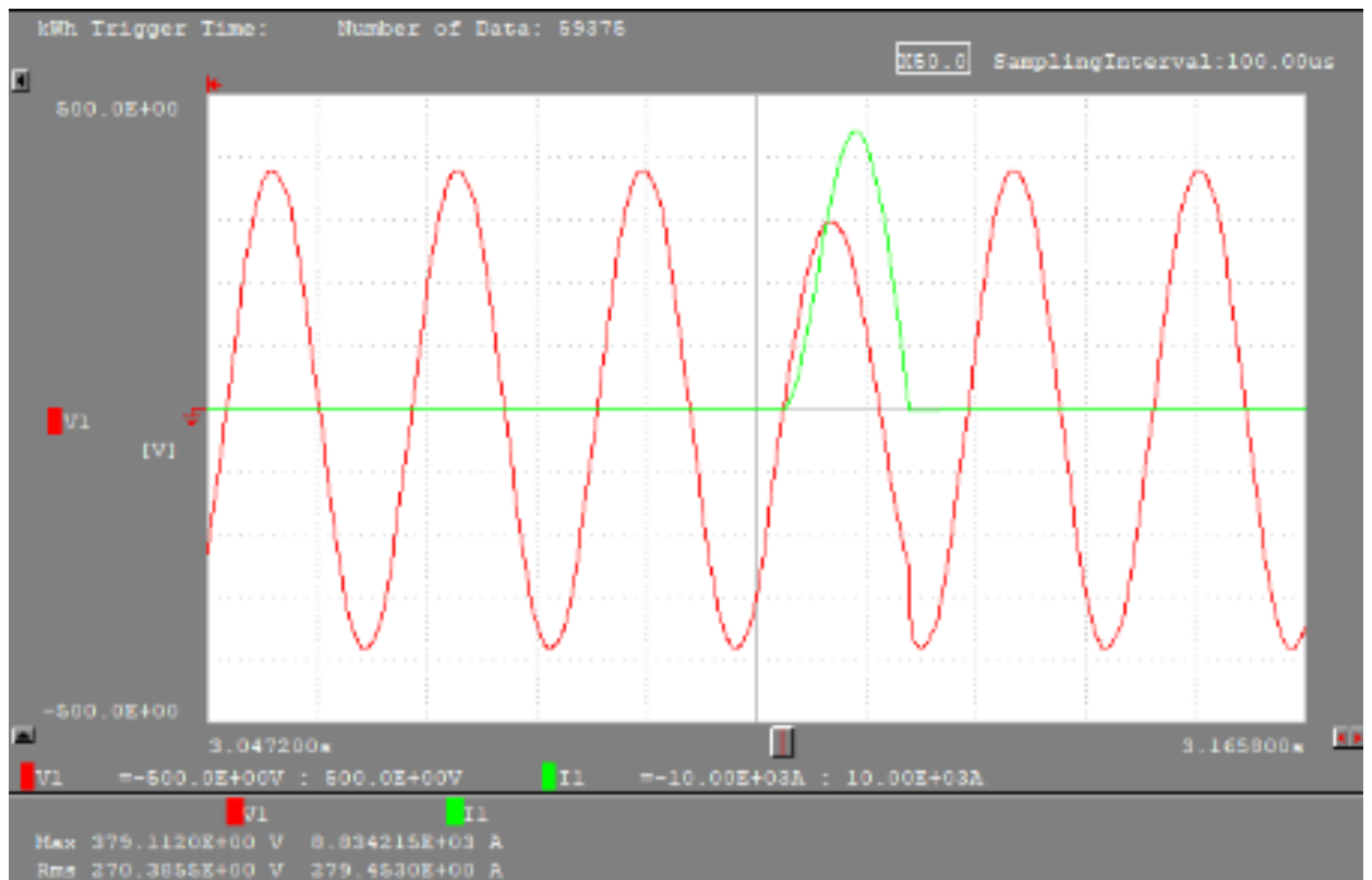
Figure 8: plot of measured test shot 1, for C6 test 1, short-circuit current carrying capacity
